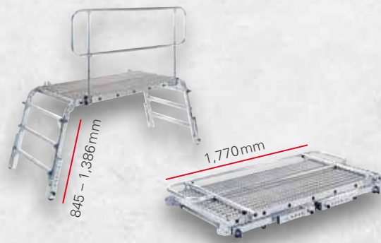
Rescue platform LRP, Dimensions: 1,770×850 mm, 49 kg, load 500 kg Art. no. 81-73-50
