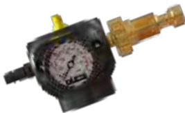
REGULATOR G3 215 PSI DIN (14.8 BAR) Piston Type Euro 5,500-0 psi / 379,2-0 bar DIN Net Weight: 3.5lb 1,6kg Part No. 22-895401DG3-12
